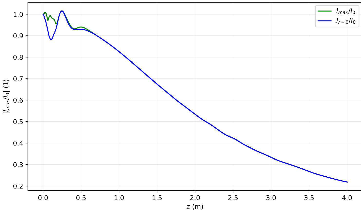
I_{\max}(x = 0, y = 0, z)/I_0 , \text{Pin}=0.1\text{Pcr} , noisy input, artificial time
